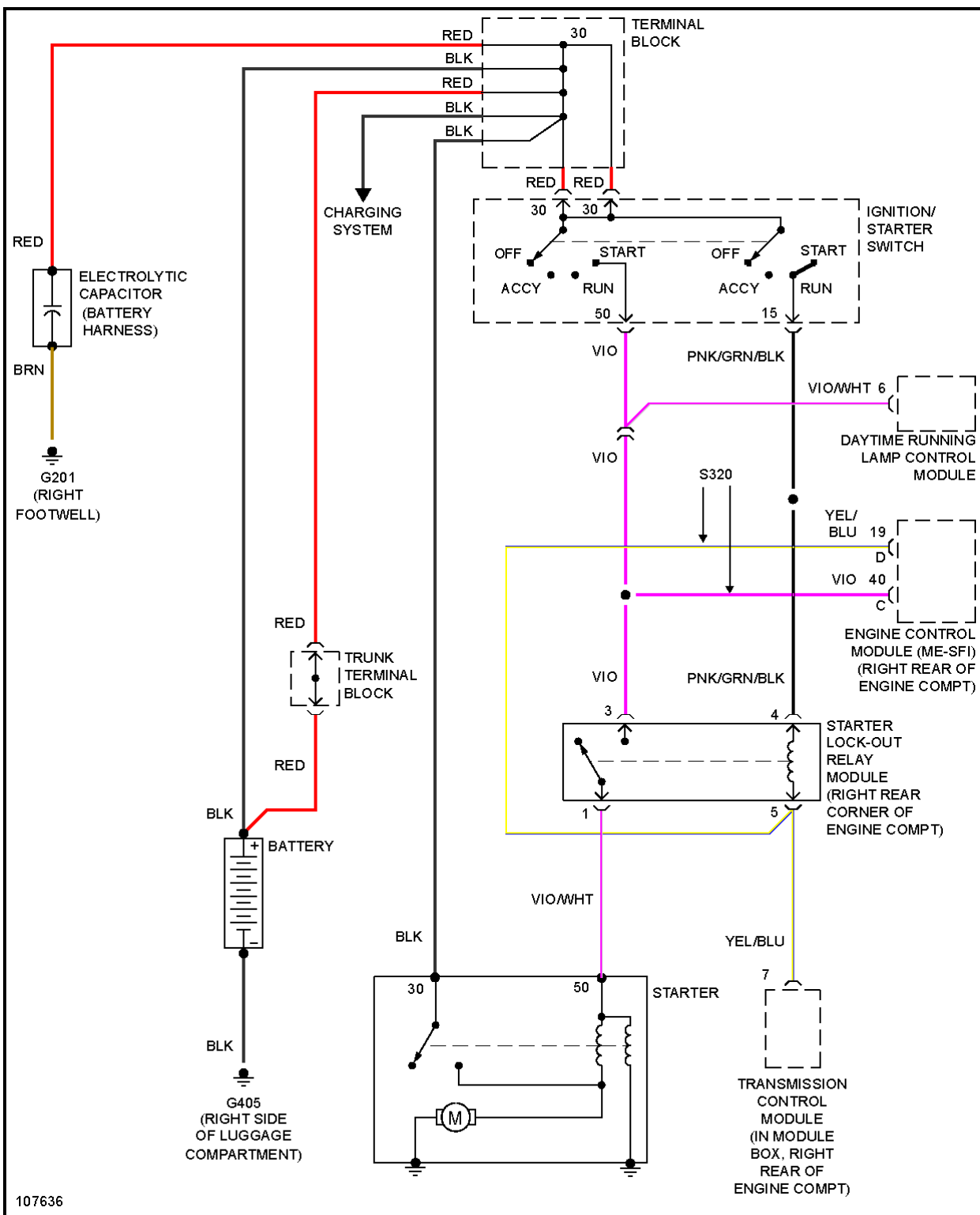
Fig. 49: Starting Circuit
